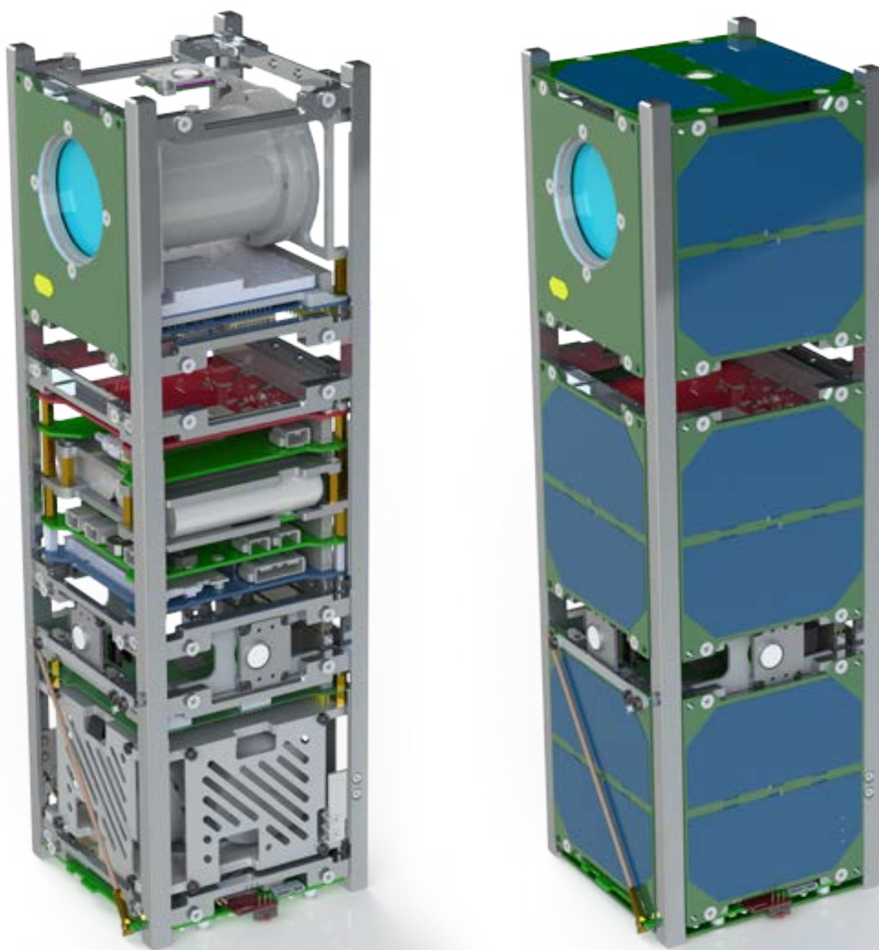
Picture 2 – SXC3 layout
